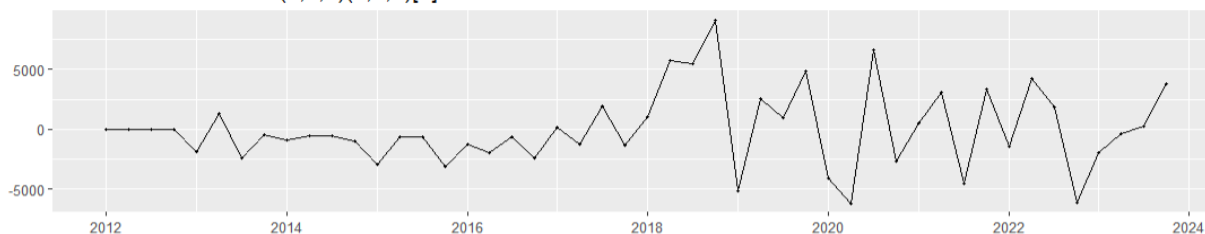
Residuals from ARIMA(1,0,0)(2,1,0)[4] with drift
