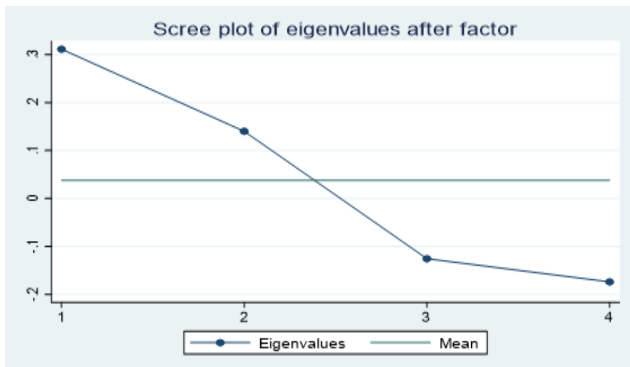
7-rasm. Samaradorlik indeksining aygen qiymati (eigenvalue)
