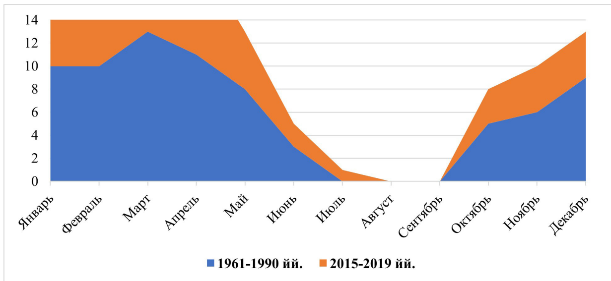
1-rasm: Boysun tumani hududida yomg'irli kunlar sonining o'zgarishining, o'rtacha ko'rsatkichlari (1961–1990-yy. va 2015–2019-yy) 4
