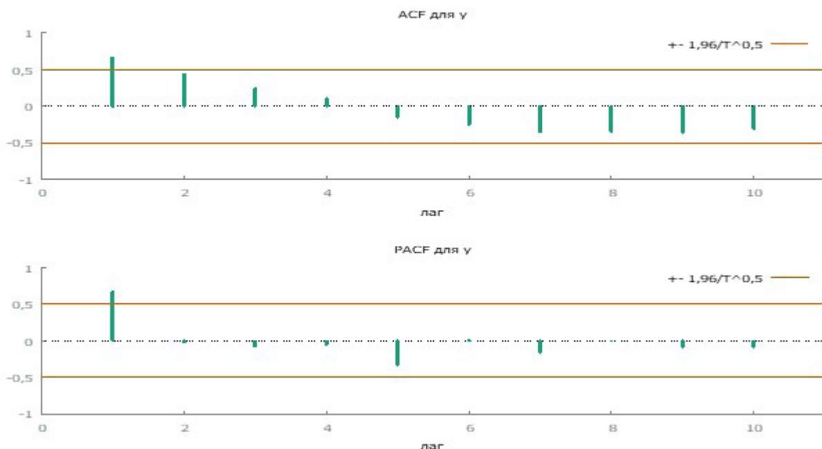
2-rasm: Vaqtli qatorning korrelogramma chizmasi 4
