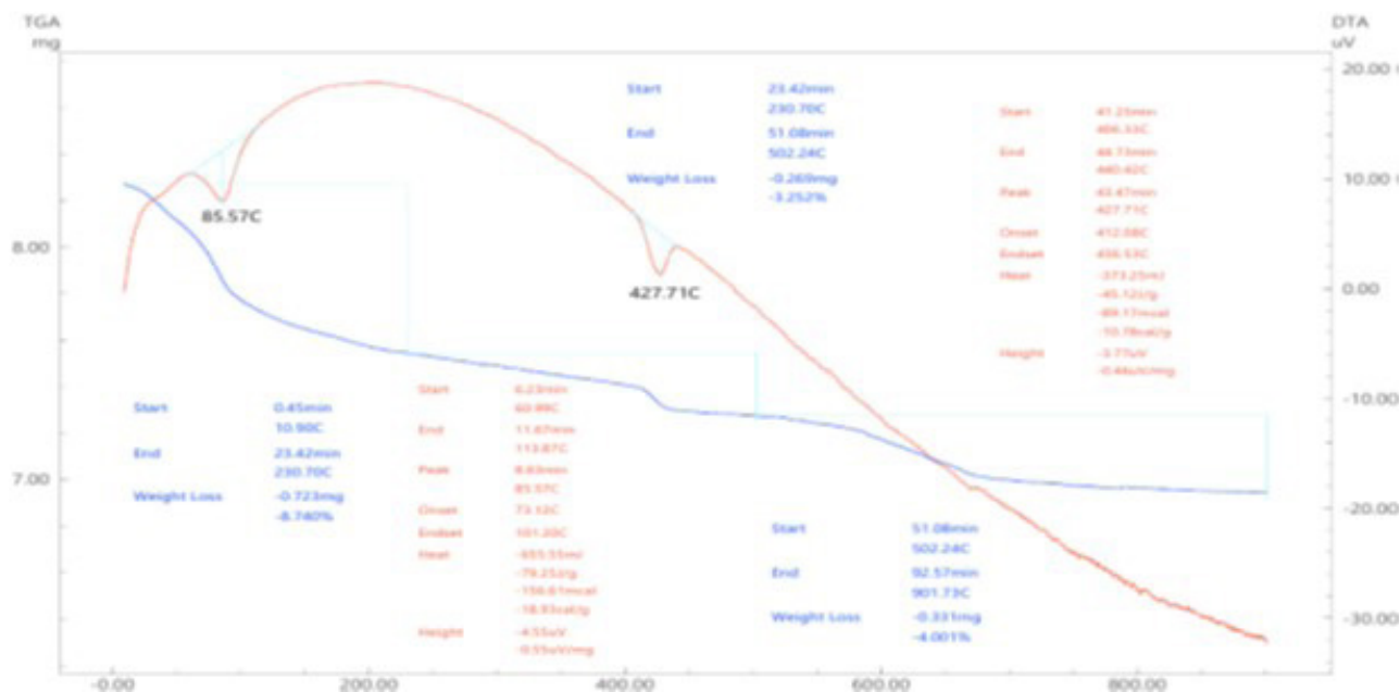
1-rasm: S-1 superplastifikator qo'shilgan beton namunalarini differensial termik tahlili
